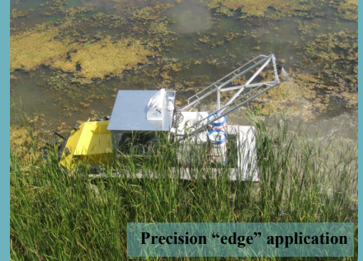
Closed-loop herbicide system
